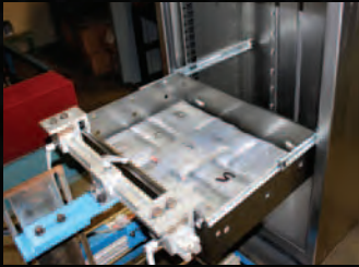
Drawer-Cycle Test
