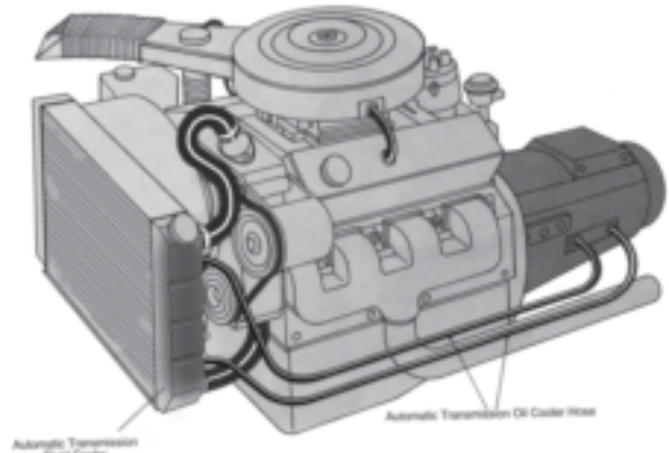
Cross-Flow Radiator
