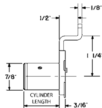
078-LB1-DW Installed Dimensions
