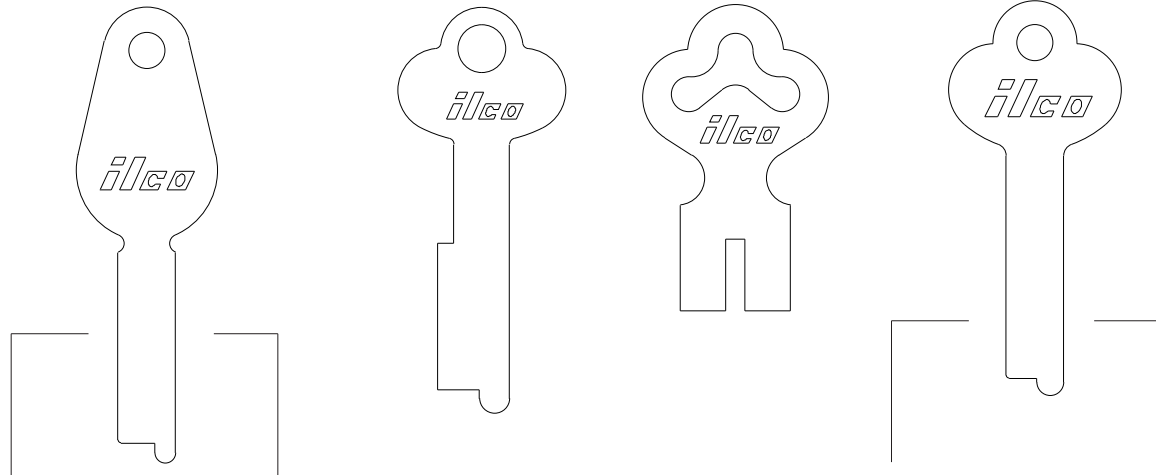
.070" - 1.8mm .300" - 7.6mm 1242 .060" - 1.5mm .300" - 7.6mm 1242L .050" - 1.3mm .375" - 9.5mm 1243D .060" - 1.5mm .575" - 14.6mm 1259 .040" - 1.0mm .300" - 7.6mm 1270 .060" - 1.5mm .300" - 7.6mm 1270H
