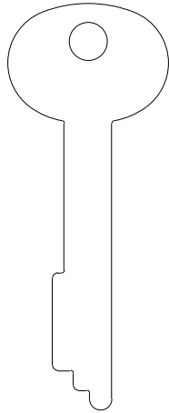
.060" - 1.5mm .340" - 8.6mm O1028AH
