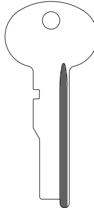
.085" - 2.2mm .320" - 8.1mm 1360G
