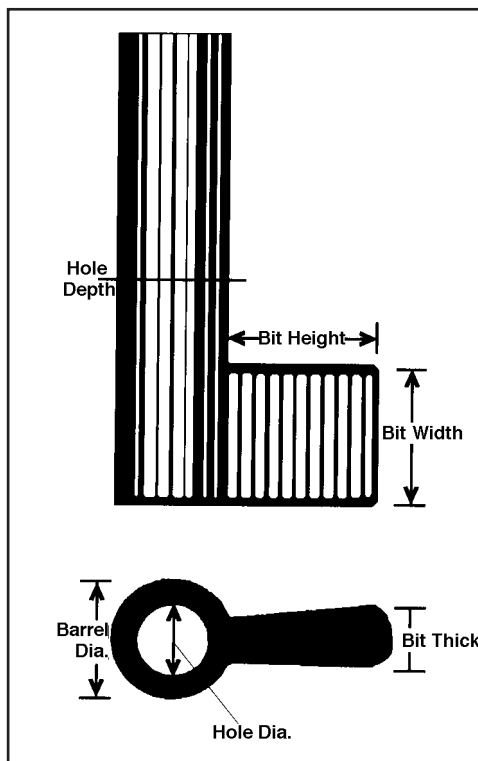
Dimensions of a Barrel Key
