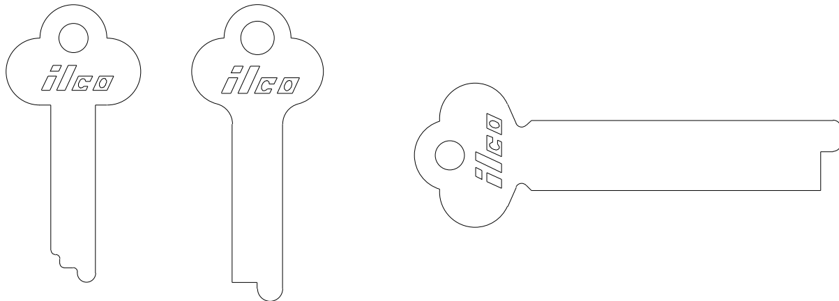
.060" - 1.5mm .325" - 8.3mm 1306 .050" - 1.3mm .375" - 9.5mm 1306A .070" - 1.8mm .525" - 13.3mm 1309
