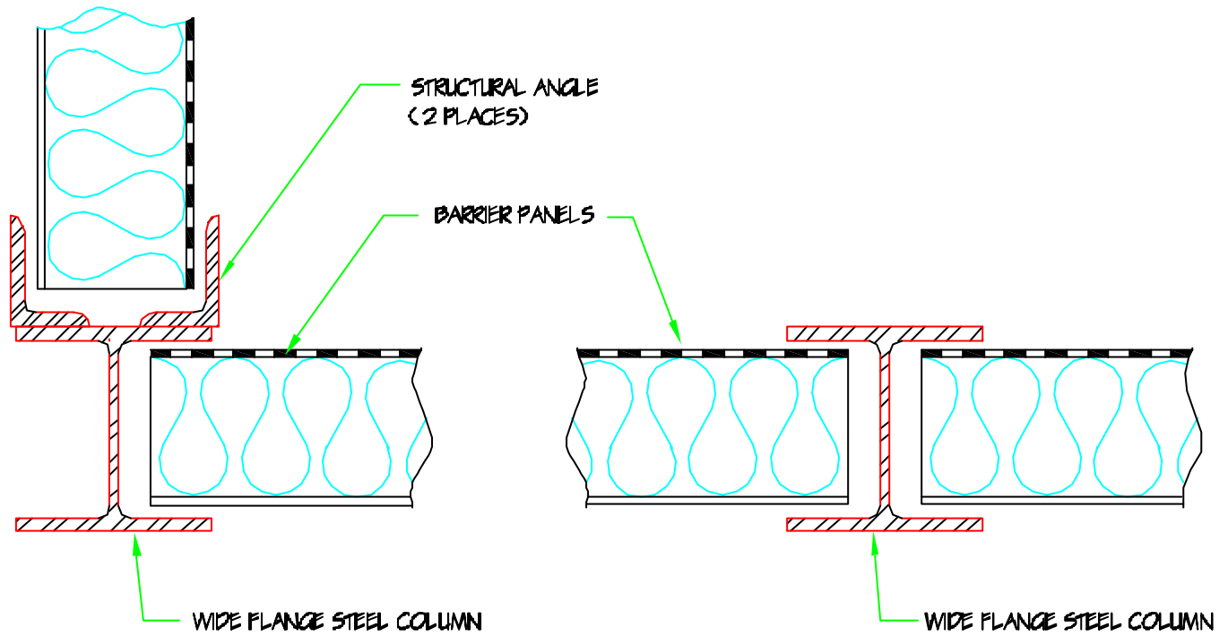
DETAIL @ CORNER
