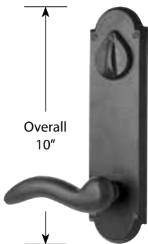
• Cody Lever with Keyed #5 Plate • Two standard 2 1/8" door preps • 5 1/2" Center to Center hole spacing
