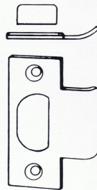
10-001 Standard "T" Strike Square Corner 1 1/8" x 2 3/4" x 3/32"
