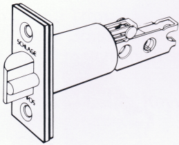
12-100 Standard Deadlatch Square Corner Front 1 1/8" Square Front 1" Housing 9/16" throw
