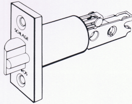
12-102 Deadlatch 1/2" Rabbeted 1 1/8" Flat Front 1" Housing 9/16"
