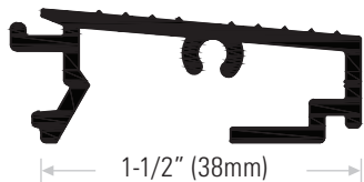
DS1112A150 Extruded aluminum mill finish. Length available: 150" (3810mm) only
