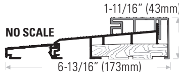
DS457 Sill shown with DS1122, 2" (51mm) extension
