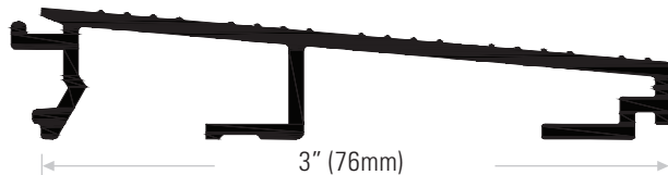
DS1113A150 Extruded aluminum mill finish. Length available: 150" (3810mm) only
