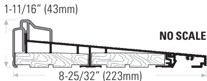
DS658 Sill shown with DS1112, 1-1/2" (38mm) extension
