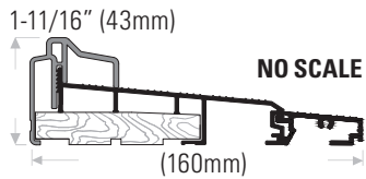
DS458 Sill shown with DS1112, 1-1/2" (38mm) extension
