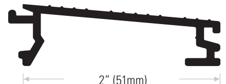
DS1128A150 Extruded aluminum mill finish. Length available: 150" (3810mm) only
