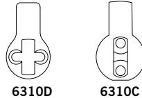
6310D 6310C SFIC cams have mounting screw holes at 12 and 6 o'clock
