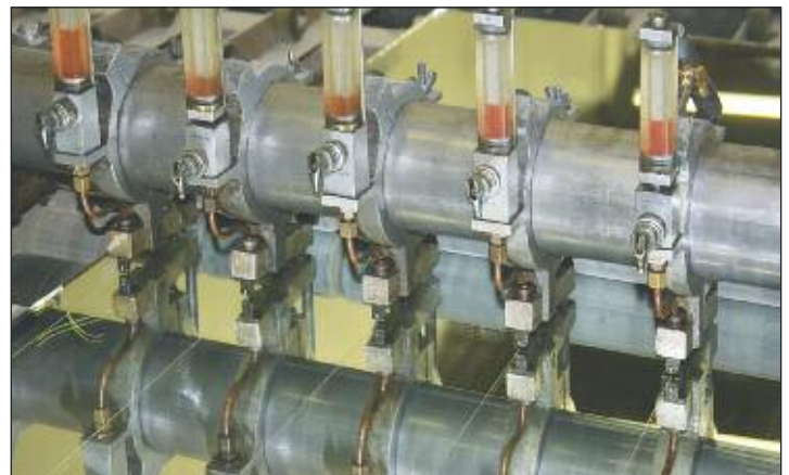
Cutting Heads on a CRL Stalter Machine in action, cutting mirror strips.
