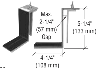
CAT. NO. SLR2
