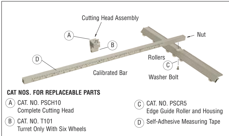
CAT. NO. PSCH10 Complete Cutting Head With Turret
