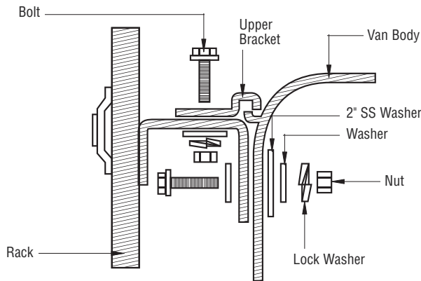
TOP MOUNT
