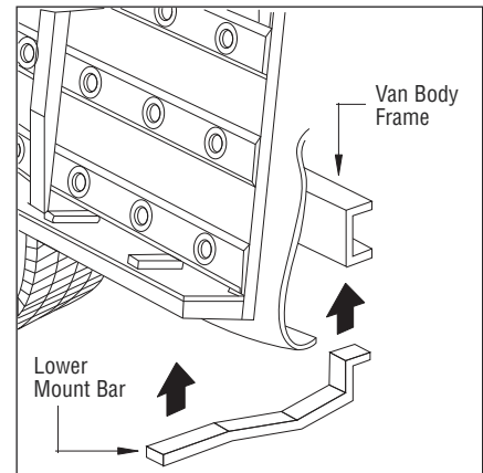
BOTTOM MOUNT
