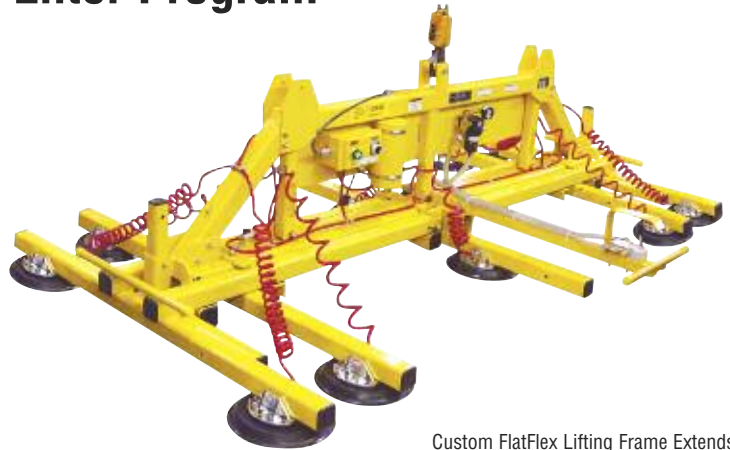
Custom FlatFlex Lifting Frame Extends to a Massive 14' (4.3 m) Length for Lifting Large Flat Sheets. Maximum Load Capacity 2500 lb. (1135 kg)
