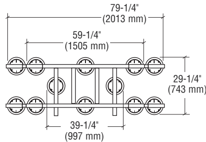
CAT. NO. CF3TA0
