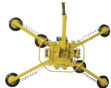
CAT. NO. MRTA611LDC
