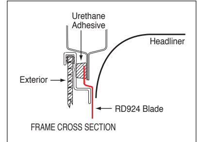
CAT. NO. RD924
