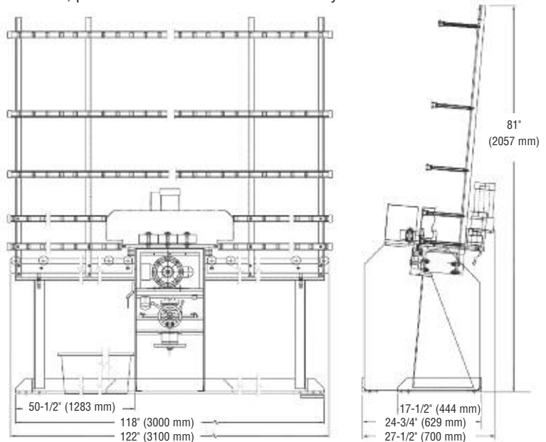
Elevation and Side View of Edger
