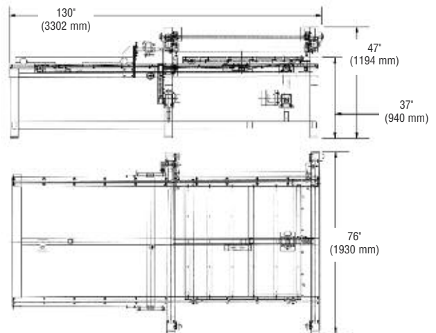
CAT. NO. SS5050FT Diagram
