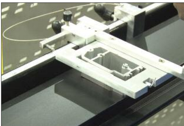
Shear Block Locator Shown with Shear Block which are purchased separately
