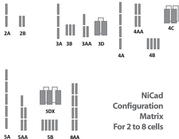
NiCAD CONFIGURATIONS
