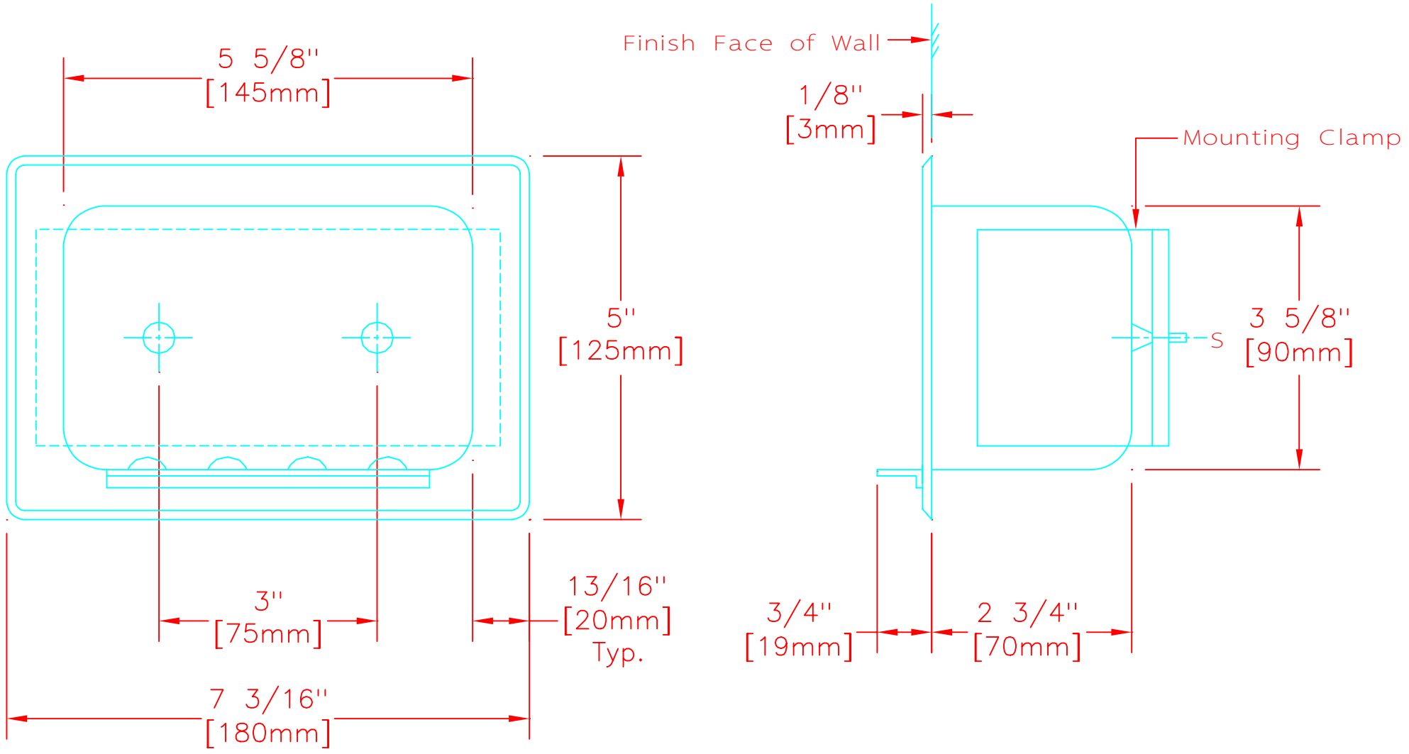
B-4380 RECESSED HEAVY-DUTY SOAP DISH (FOR STUD WALLS)
