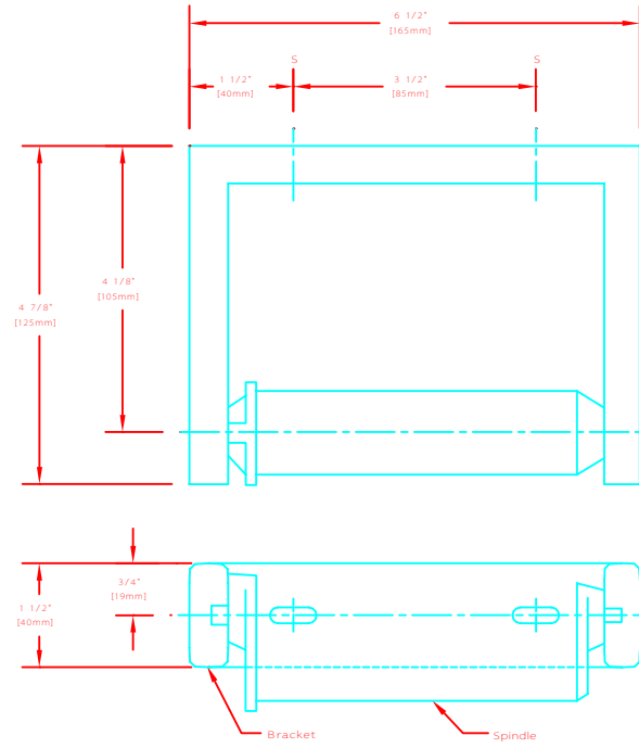
B-273.DWG SINGLE-ROLL TOILET TISSUE DISPENSER WITH CONTROLLED DELIVERY
