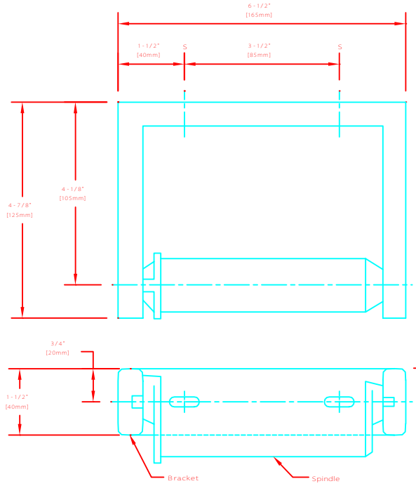
SINGLE-ROLL TOILET TISSUE DISPENSER B-2730.DWG
