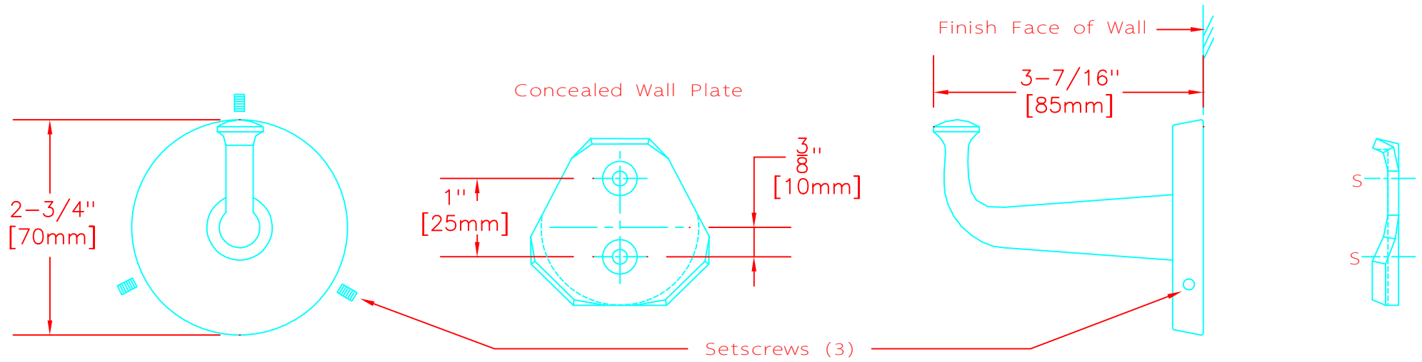
HEAVY-DUTY ROBE HOOK WITH CONCEALED MOUNTING B-2116.DWG
