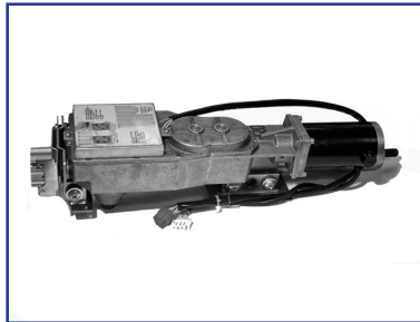
Rebuilt Operators: 30-10-001R SM 300 OHC 35-10-001R SM 400 RH OHC 35-10-002R SM 400 LH OHC 35-10-003R SM 405 RH OHC 35-10-004R SM 405 LH OHC
