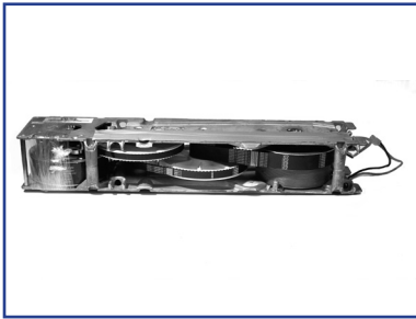
24-10-173233R Navig-Aider Operator Rebuilt
