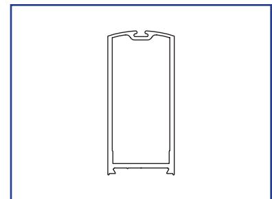
US01-0409-LLCL Medium Stile Single Fuzz, Nose Rail US01-0409-LLDB Medium Stile Single Fuzz, Nose Rail
