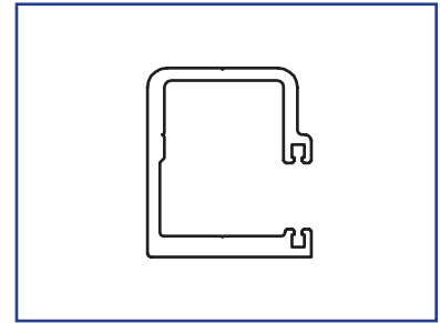
50-01-100 G Channel 50-04-146 42" G Channel 50-04-147 48" G Channel
