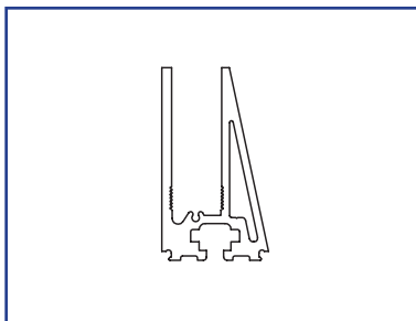
US01-0547-LLCL CGL Shoe US010547-LLDB CGL Shoe
