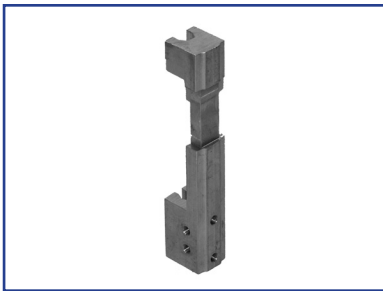
US04-0537-02 Spring GuideBlock US04-0641-01 Guide Block Shim 40-09-200 Screw, 1/4-20" x 3/4" 52-09-004 Screw, 1/4-20" x 1"
