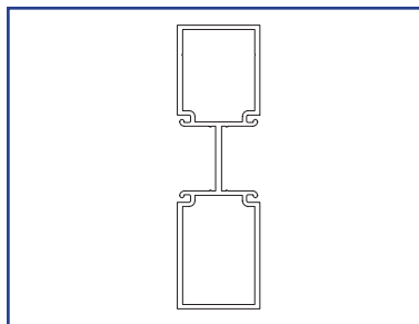
US01-0979-LLCL Redesigned 6" Jamb Tube US01-0979-LLDB Redesigned 6" Jamb Tube
