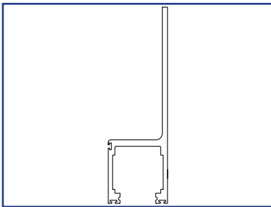
US01-0292-LLCL Telescopic UniSlide, Carrier US01-0292-LLDB Telescopic UniSlide, Carrier
