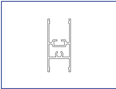
US01-0412-LLCL 4" Bottom Top Rail US01-0412-LLDB 4" Bottom Top Rail
