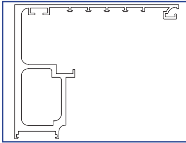
US01-1261-LLCL UniSlide (plankless heavy beam)
