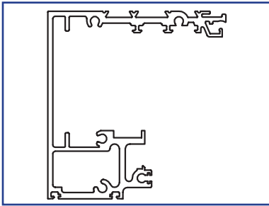
US01-0585-LLCL ICU, Beam US01-0585-LLDB ICU, Beam
