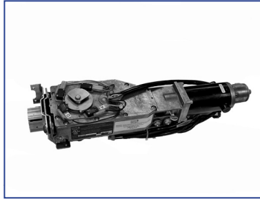
Operator: US05-0583-21 Surface Mounted Spring #1 US05-0583-22 Surface Mounted Spring #2 US05-0583-21R Surface Mounted Spring #1, Rebuilt US05-0583-22R Surface Mounted Spring #2, Rebuilt
