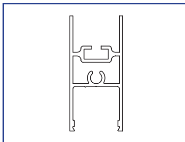
US01-0455-LLCL 2 3/16" Top Rail US01-0455-LLDB 2 3/16" Top Rail
