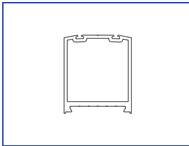
US01-1632-LLCL Narrow Stile Double Fuzz, Nose Rail, Standard Wall US01-1632-LLDB Narrow Stile Double Fuzz, Nose Rail, Standard Wall
