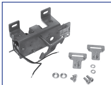
04-02-692065 Lock, Electric AMD/EMD-2 Fail Safe, BiPart 04-02-692068 Lock, Electric AMD-RH/EMD-LH Fail/Safe 04-02-692069 Lock, Electric AMD-LH/EMD-RH Fail/Safe
