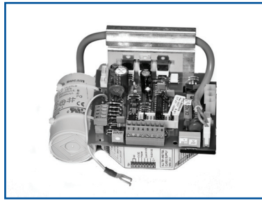
600085R PowerSwing Control Board, CSDA Rebuilt
