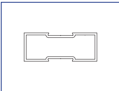
US01-0432-LLCL Double Dovetail Jamb Tube US01-0432-LLDB Double Dovetail Jamb Tube
