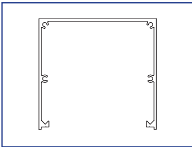
US01-0594-LLCL Swingmaster Bottom Load, Header US01-0594-LLDB Swingmaster Bottom Load, Header
