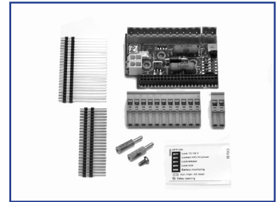
1003554 SW100 Security & Impulse Kit, EXU-SI *Use with battery back-up, electric lock and open/close ratchet impulse.
