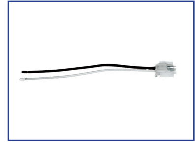
US02-0583-18 120V, Male 2-pin Harness
