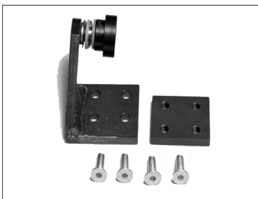
US05-0568-01 Trackless ICU Door Foot, LH
