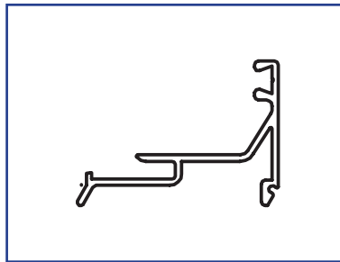
US01-0420-LLCL 5/8" and 1" Gutter US01-0420-LLDB 5/8" and 1" Gutter
