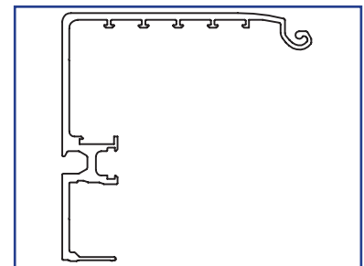
US01-0295-LLMF UniSlide Beam *
