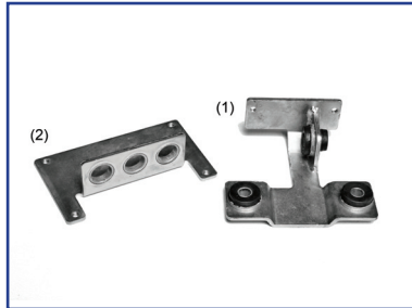
30-04-005 Mount, Operator, Hinge Side (1) 30-04-006 Mount, Operator, Hinge Side (2)
