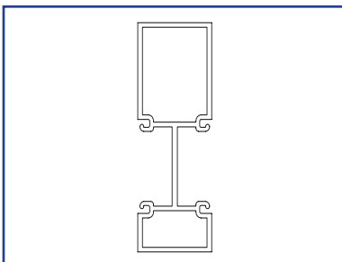
US01-0934-LLCL Redesigned Mullion Tube US01-0924-LLDB Redesigned Mullion Tube
