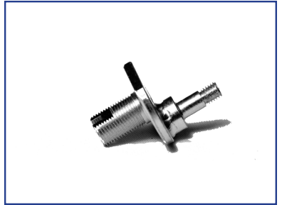
12-03-013 Eccentric for ICU Roller
