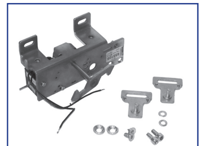
04-02-692064 Lock, Electric AMD/EMD-2 Fail Secure, BiPart 04-02-692066 Lock, Electric AMD-RH/EMD-LH Fail Secure 04-02-692067 Lock, Electric AMD-LH/EMD-RH Fail Secure
