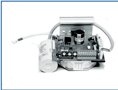
1004204 PowerSwing Control Board, CSDB 1004204R PowerSwing Control Board, CSDB Rebuilt * Refer to Technical Bulletin M155 for additional information
