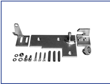
12-15-104 Pivot and Guide, A/L, RH, Kit
