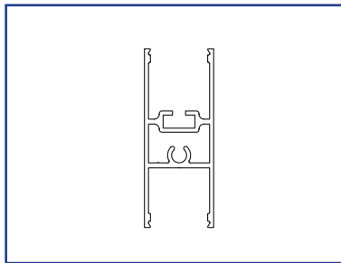
US01-0567-LLCL 4 1/2" Bottom Rail US01-0567-LLDB 4 1/2" Bottom Rail
