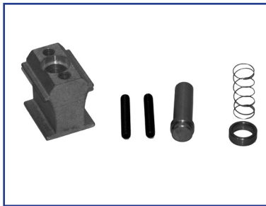
US05-0626-01 Assembly Lock Pin
