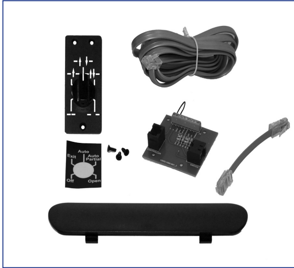
US15-1500-08 Retrofit Kit, UniSlide, 5 Pos Switch *May require additional parts for some applications (i.e., remote mount, over size doors)
