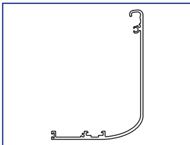
US01-0296-LLCL UniSlide Cover
