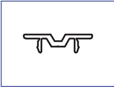
US01-0517-LLMF Resilience Threshold Filler
