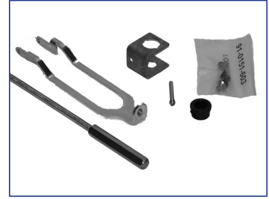
50-06-110/HD Assembly, Lock Rod, 3-Point Converter
