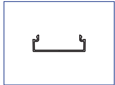
US01-0299-LLCL UniSlide Square Plank Cap US01-0299-LLDB UniSlide Square Plank Cap
