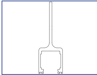
US01-1263-LLCL Plankless UniSlide, Carrier US01-1263-LLDB Plankless UniSlide, Carrier
