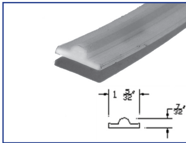
18-20-002 Track, C Series
