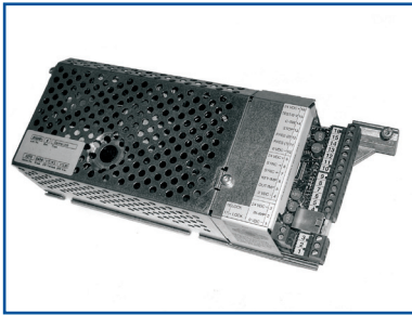
600091 UniSlide Control 600091R UniSlide Control Rebuilt
