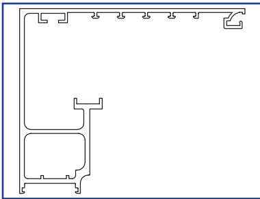
US01-1260-LLCL UniSlide (plankless beam) Standard
