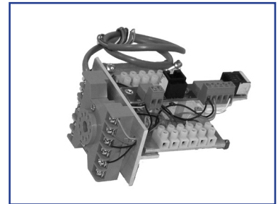
US05-0521-01 Interlock Interface, Assembly
