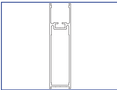
US01-0416-LLCL 7" Bottom Rail US01-0416-LLDB 7" Bottom Rail
