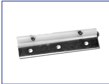
US05-0553-01 ICU Dampener Assembly, LH
