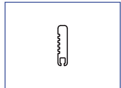
US01-0685-LLDB Brush Holder Concealed Sweep
