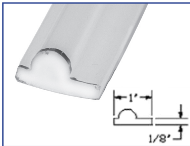
04-21-701239 Track, Extrusion, Roller, AMD/EMD, Per Foot
