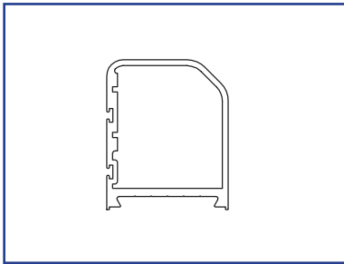
US01-1633-LLCL Narrow Stile Besam Rail, Standard Wall US01-1633-LLDB Narrow Stile Besam Rail, Standard Wall
